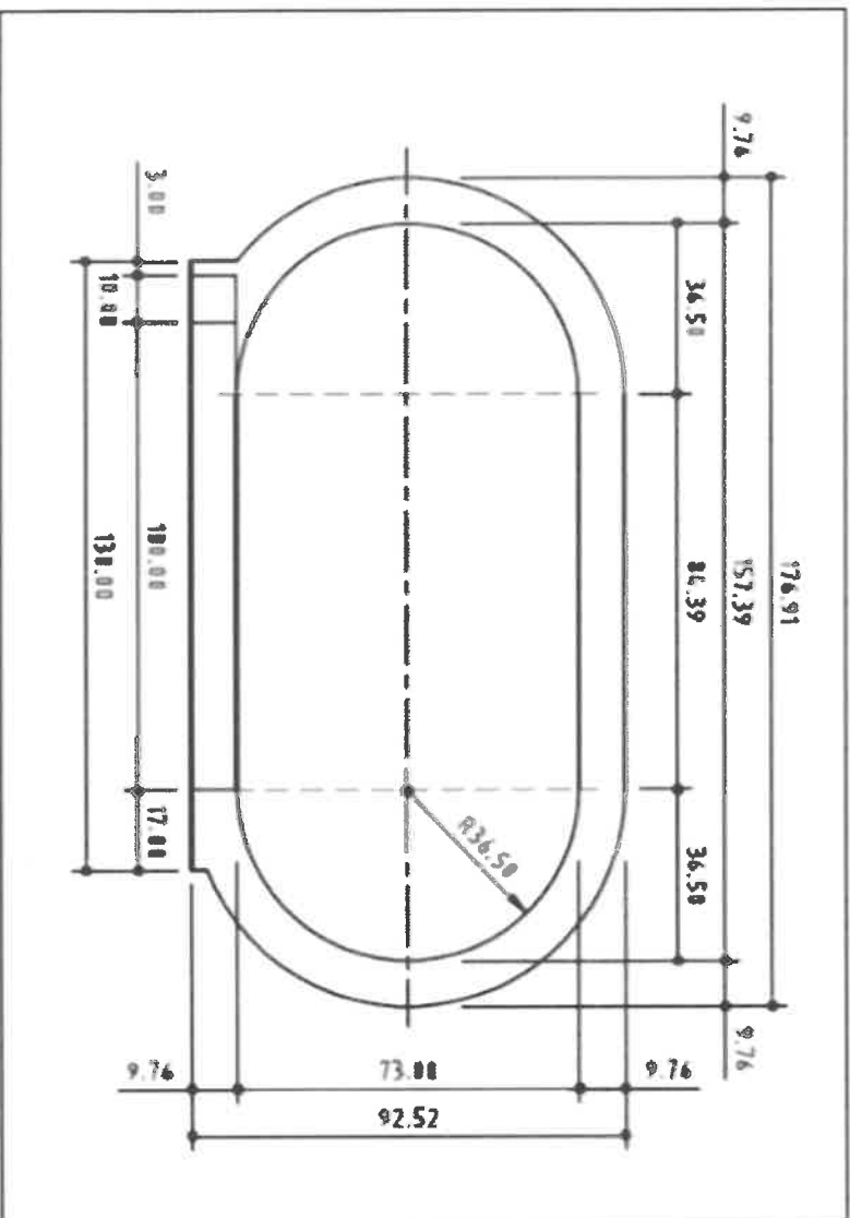
Figure 1.2.3a - Shape and dimensions of the 400m Standard Track (Radius 36.50m) (Dimensions in m)
