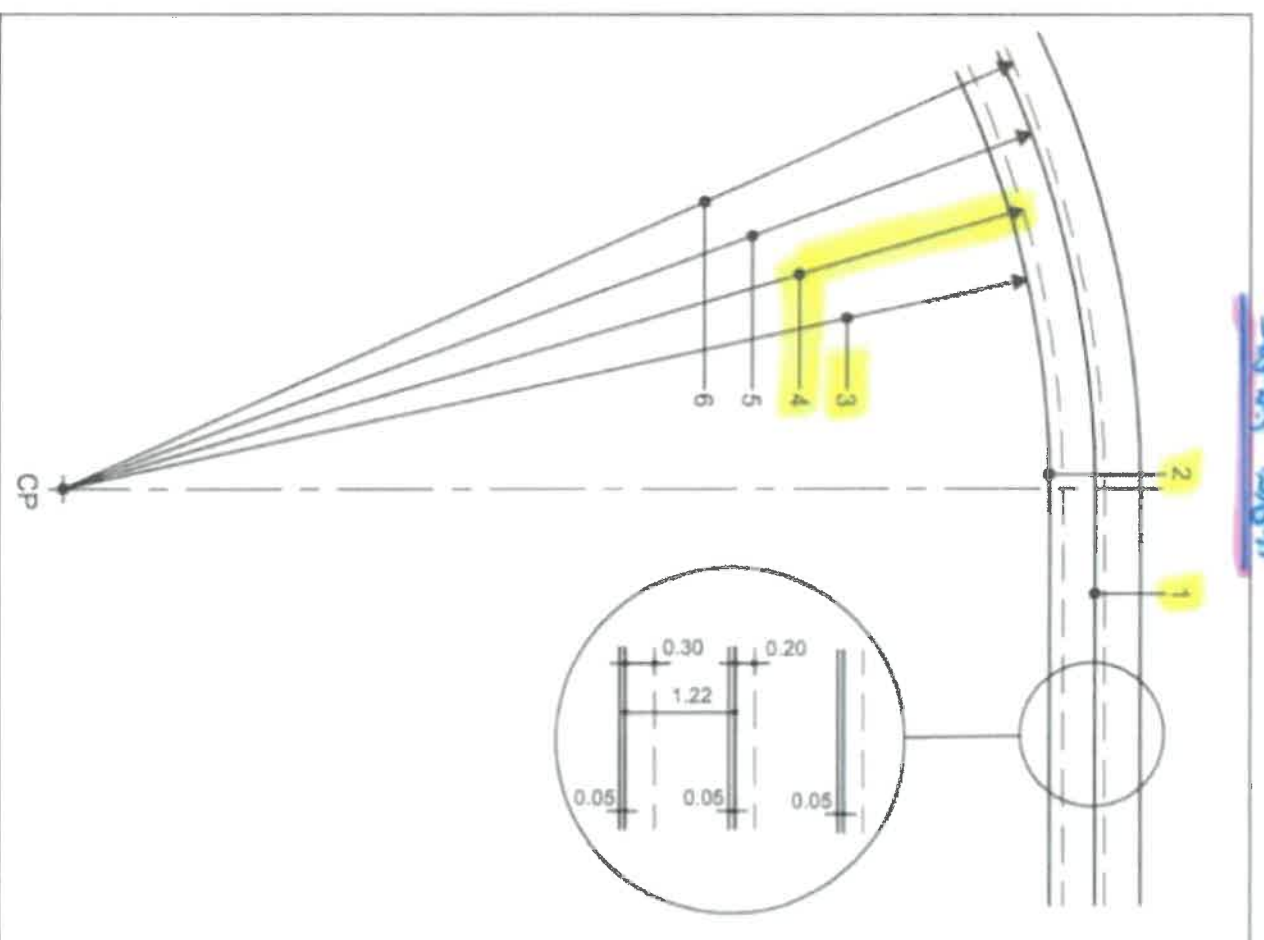
Figure 2.2.1b - Calculation of the track length of the 400m Standard Track (Dimensions in m)
